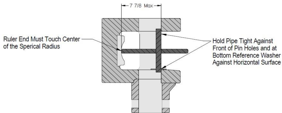
F-Type Floating Yoke or Endcap
