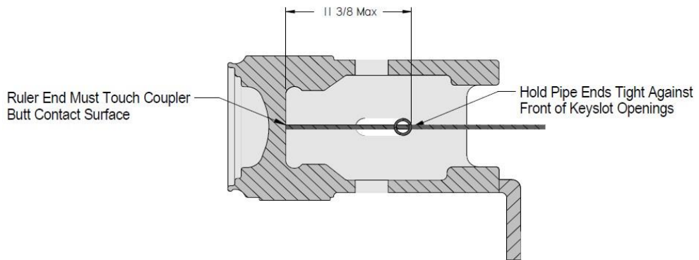
E-Type Floating Yoke or Endcap
